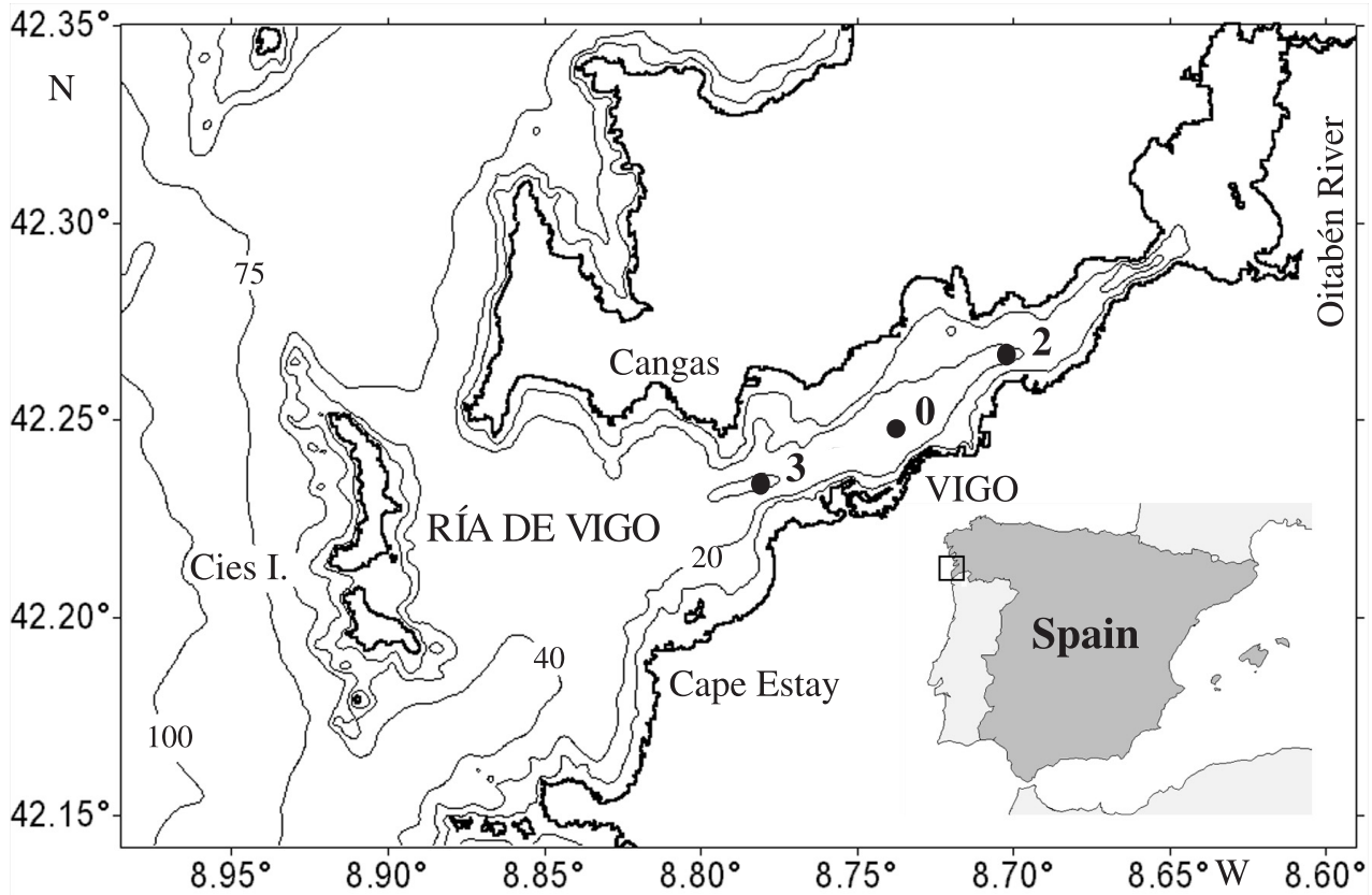
FIG. 1. – The Ría de Vigo and the position of three stations 3, 0 and 2 sampled between February 1988-1989. Isobaths in metres.
