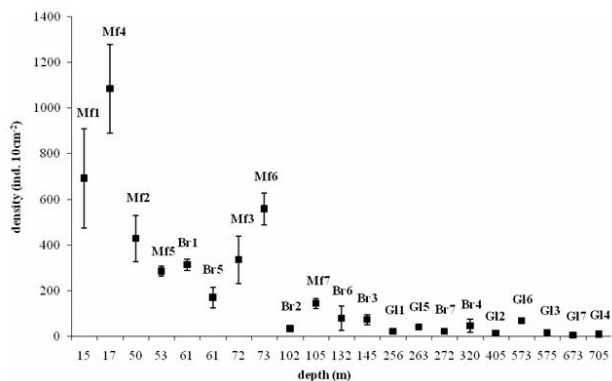
FIG. 2. – Total meiofauna density (±SE) versus depth (m) in the three study areas.
