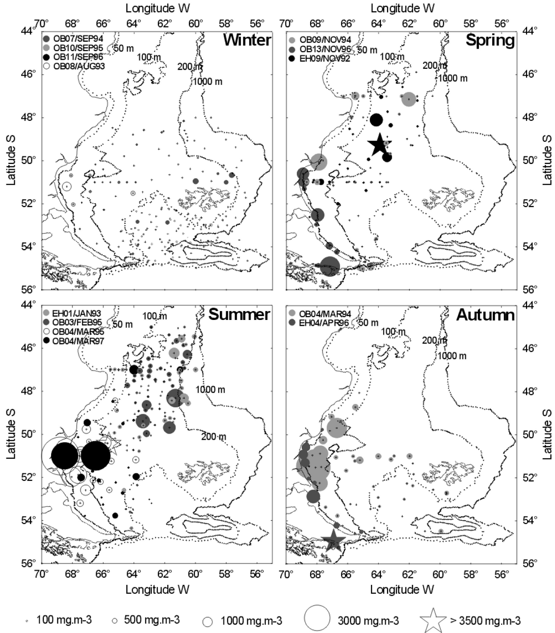
FIG. 2. – Seasonal synoptic distribution of total zooplankton biomass ( \text{mg WW m}^{-3} ) in Argentinian waters off southern Patagonia recorded during the several surveys listed in Table I.
