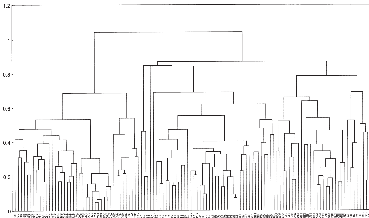
Fig. 2. – Cluster analysis performed on the matrix of fish species composition standardized to 1 h of trawling (1-r; UPGMA). Codes of the samples indicate mean depth of the haul.
