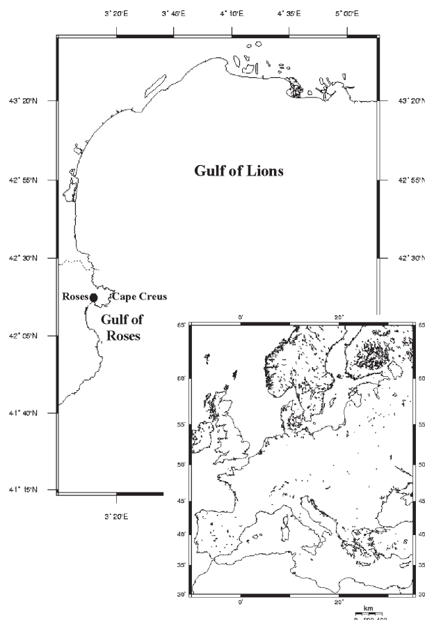
FIG. 1. – Location of the study area (Gulf of Lions and Gulf of Roses; NW Mediterranean) showing the fishing port of Roses where landings are recorded monthly and length sampling was conducted.
