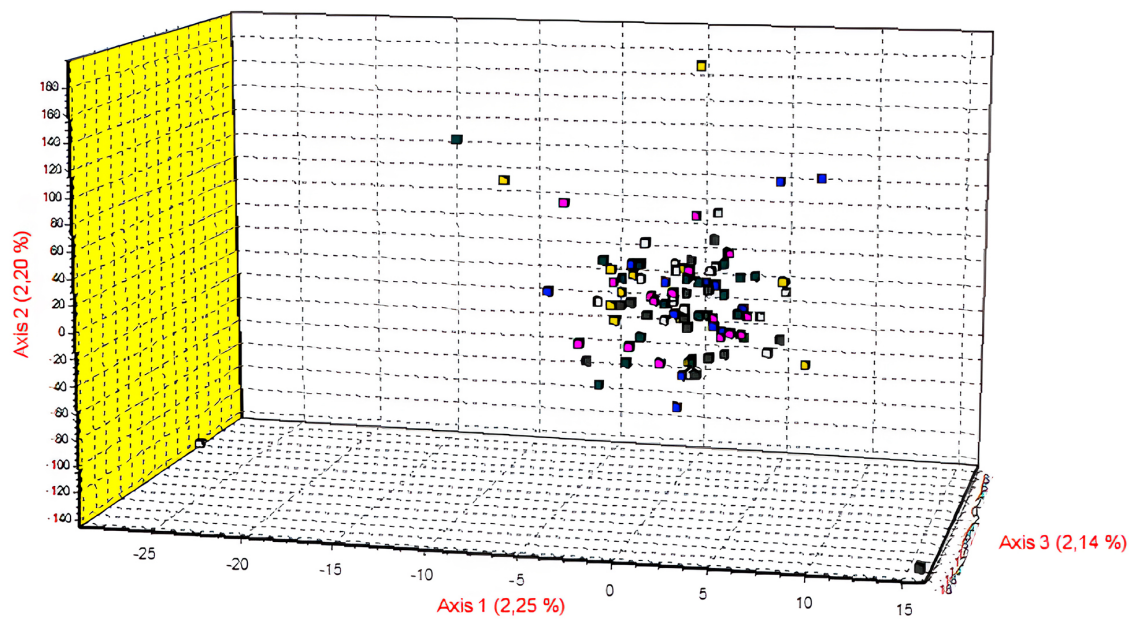
Figure S1. – FCA of the 97 lobsters analysed. No structure is apparent when the elementary information is the individual.
