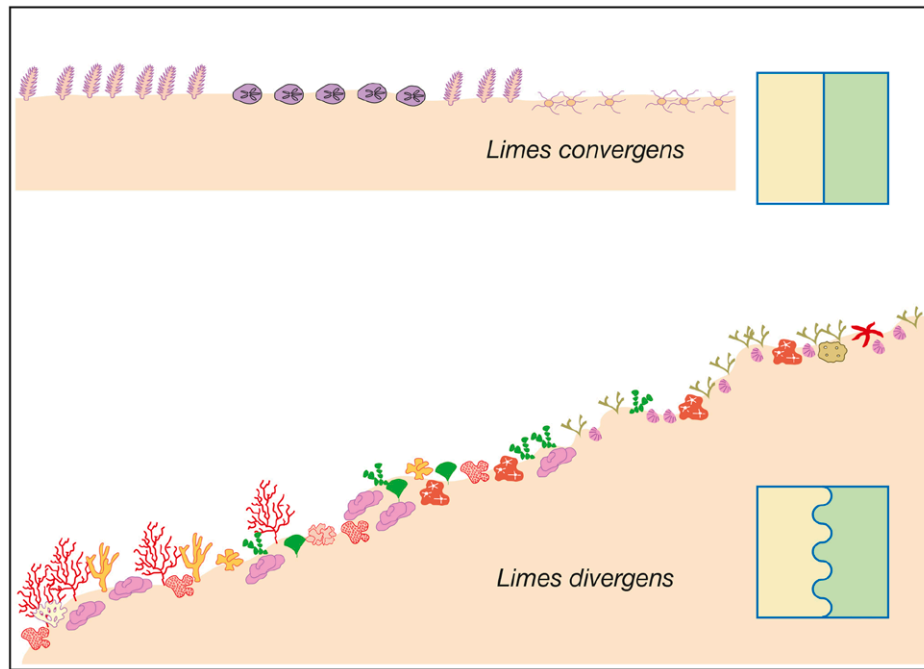
Fig. 1. – Different benthic profiles with linear, contrasting limits and low fractal limits ( limes convergens ) or sinuous, diffuse limits with a high fractal index ( limes divergens ). Redrawn from van Leeuwen (1966).
