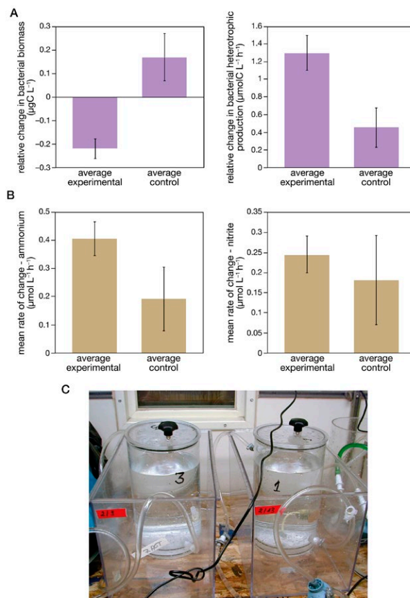
Fig. 6. – Experiments with the demosponge Stylocordyla chupachups (C) showing that sponges feed on bacteria, as bacterial abundance decreases (A left) and bacteria production increases (A right), but also enhance inorganic nutrient enrichment of water with both ammonium (B left) and nitrite (B right), increasing incubation time.
