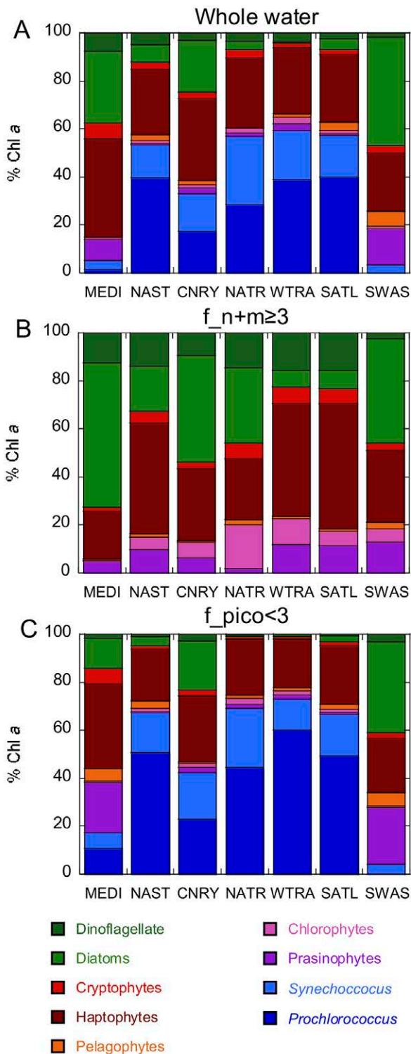
Fig. 7. – Percentage contribution of the chemotaxonomic phytoplankton groups to Chl a_{tot} for the whole community (A), the nano+microphytoplankton ( f_{n+m \geq 3} ) size class (B), and the picoplankton ( f_{pico < 3} ) size class (C).
