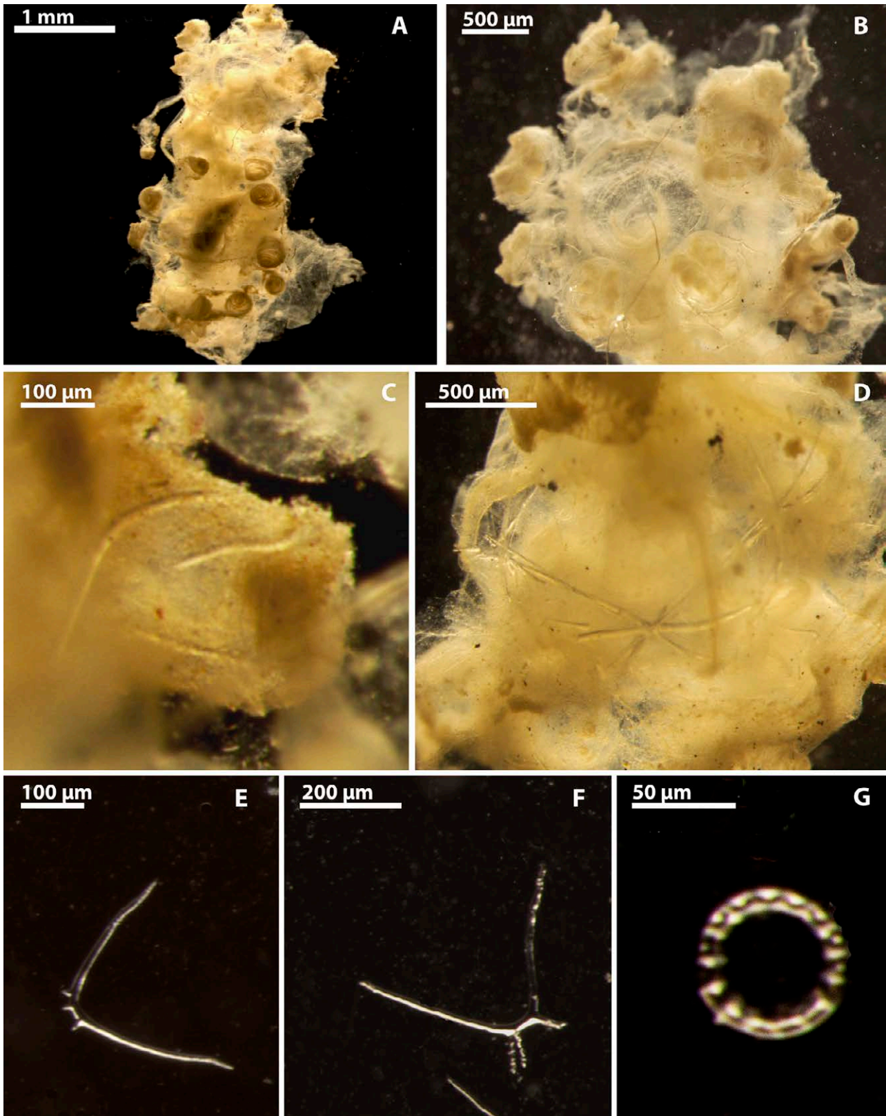
Fig. 12. – Penilpidia ludwigi characteristic. A, general view; B, oral region detail; C, tentacle ossicles; D, interlinked pieces of the calcareous ring; E, F, pieces of the calcareous ring G, wheel from skin.
