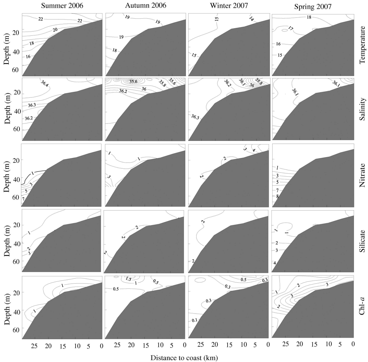
FIG. 5. – Vertical distributions of temperature (°C), salinity, chl- a ( \mu\text{g dm}^{-3} ), nitrate ( \mu\text{M} ) and silicate ( \mu\text{M} ) at transect F off Guadalquivir River during the summer, autumn, winter and spring cruises
