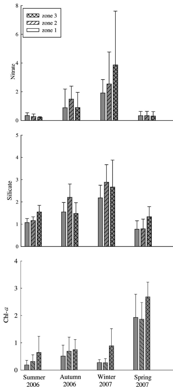
FIG. 7. – Seasonal average values of nitrate ( \mu\text{M} ), silicate ( \mu\text{M} ) and chl- a ( \mu\text{g dm}^{-3} ) between the sea surface and nitracline depth for the three zones. Zone 1 corresponds to the oceanic area while zones 2 and 3 indicate the south and north regions respectively (Fig. 1).
