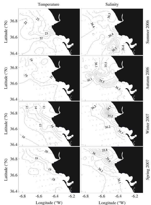
Fig. 2. – Horizontal distributions of sea surface temperature (°C) and salinity in the Gulf of Cádiz during the summer, autumn, winter and spring cruises.
