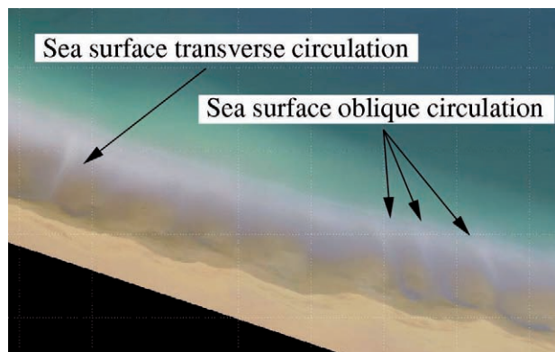
FIG. 6. – Sea-surface transverse and oblique circulations, 3 March 2004.
