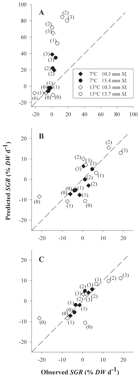
FIG. 3. – Predicted specific growth rate ( SGR , % DW d^{-1} ) over the experimental period for the four growth trials based on feeding strike frequency and bioenergetic budget compared to observed SGR . A: No adjustment of parameters (base case); B: Feeding activity in all treatments reduced to 12%, note different scaling on x- and y-axes; C: Assimilation efficiency reduced; Numbers denote prey environment: (0) no, (1) small, (2) medium, (3) large prey. Dashed line indicates 1:1 relationship.
