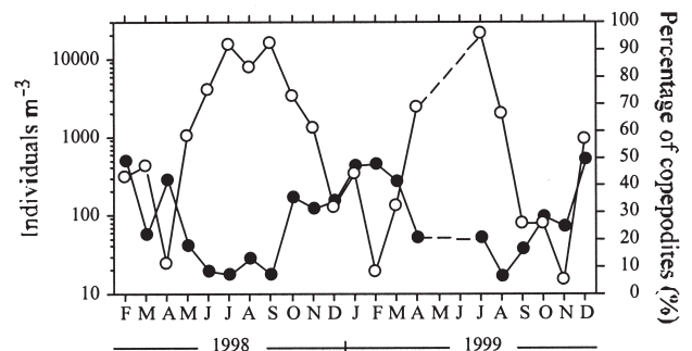
FIG. 3. – Temporal variations in Acartia bifilosa densities (blank circles) and in percentage of A. bifilosa copepodites (filled circles) at salinity 26 in the Urdaibai estuary from February 1998 to December 1999.
