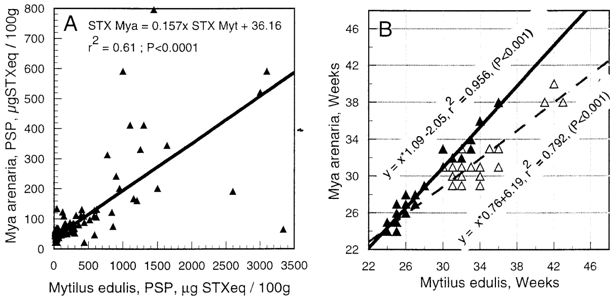
FIG. 3. – A, Relationship between M. edulis PSP toxicity and M. arenaria PSP toxicity. B, ▲: Relationship between the first date at which the PSP in the mussels ( Mytilus ) and in the clams ( Mya ) exceeds the regulatory closing level of 80 \mu\text{g STX eq}/100 \text{g} tissue; △: Relationship between the first date at which toxicity of the mussels and clams falls below this level of 80 \mu\text{g STX eq}/100 \text{g} tissue. Weeks refers to the number of weeks from the beginning of the year.
