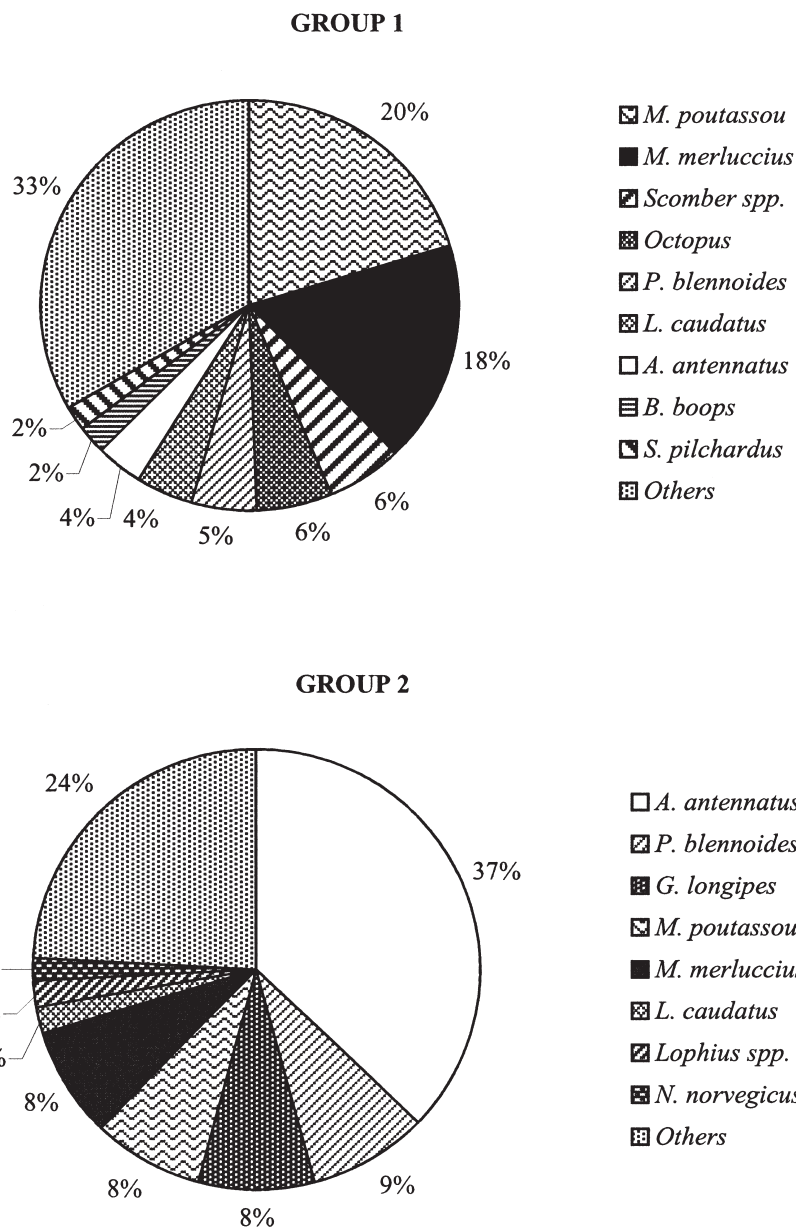
FIG. 6. – Catch species composition as a percentage for Vessel Group 1 (upper) and Vessel Group 2 (lower). Data for the Santa Pola red shrimp fleet landings 1992-1999.
