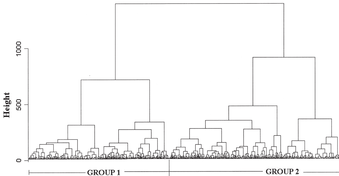
FIG. 5. – Results of the Agglomerative Hierarchical Clustering on the specific landing composition for the red shrimp fleet in the port of Santa Pola.
