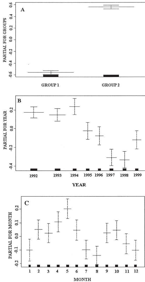
FIG. 7. – Results of Main Effects Model. Each plot represents the contribution of the corresponding variable to the fitted linear predictor for Vessel Groups (A), year (B) and month (C). The fitted values are adjusted to average zero and the dashed bars indicate S.D. The width of the solid bars at the base of the plots is proportional to the number of observations at each level of the factors.
