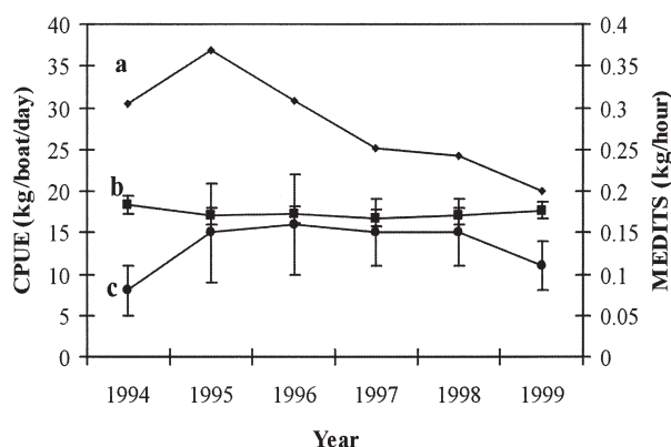
FIG. 9. – Comparison between uncorrected CPUE (a), corrected CPUE (b), and the MEDITS Survey abundance index (c). Data for the Santa Pola red shrimp fleet landings 1994-1999 and MEDITS Survey data 1994-1999.
