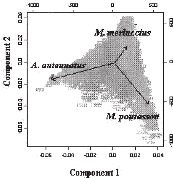
FIG. 4. – Principal Components Analysis (PCA) results; biplot from the PCA showing the grouping of the species. Data for the Santa Pola red shrimp fleet landings 1992-1999.
