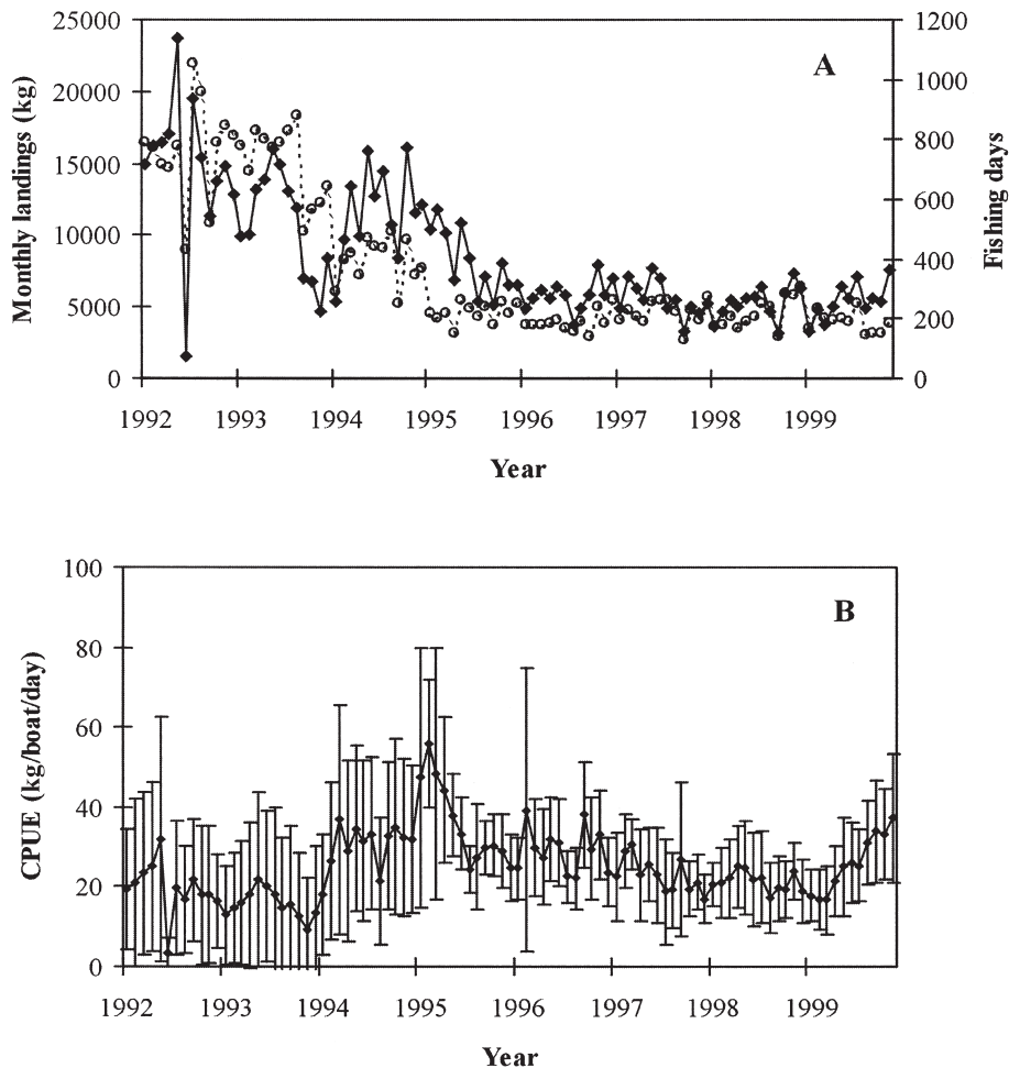
FIG. 3. – Monthly landings (solid line) and effort (dashed line) (A) and uncorrected CPUE (kg/boat/day) evolution (B) for Aristeus antennatus in the port of Santa Pola during 1992-1999. Data from RIM-IEO for the shrimp trawl fleet.
