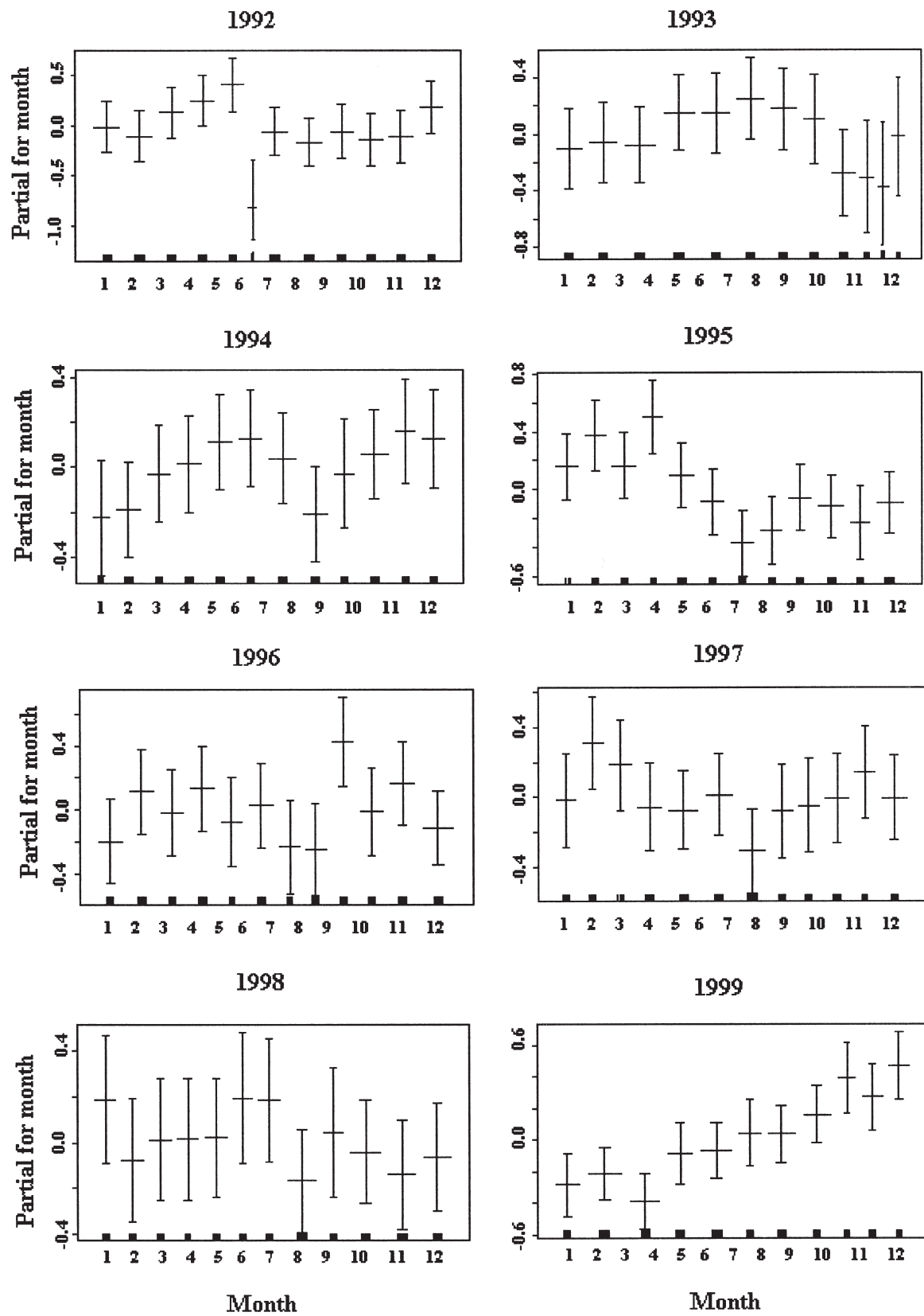
FIG. 8. – Evolution of the relative monthly catch rates by year; GLM Main Effects Model: The fitted values are adjusted to average zero and the dashed bars indicate S.D. The width of the solid bars at the base of the plots is proportional to the number of observations at each level of the factors.
