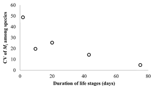
Fig. 2. – Decrement in the coefficient variation (CV) of the natural mortality at age ( M_i ) among the brown ( F. californiensis ), blue ( L. stylirostris ) and white ( L. vannamei ) shrimps in relation to the duration of their life stages (not including egg and pre-adult stage).
