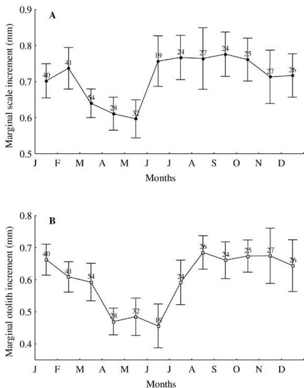
Fig. 2. – Mean monthly marginal increments of scales (A) and otoliths (B) of Spondyliosoma cantharus from the Gulf of Tunis. The errors bars represent ± standard error with monthly sample size above.
